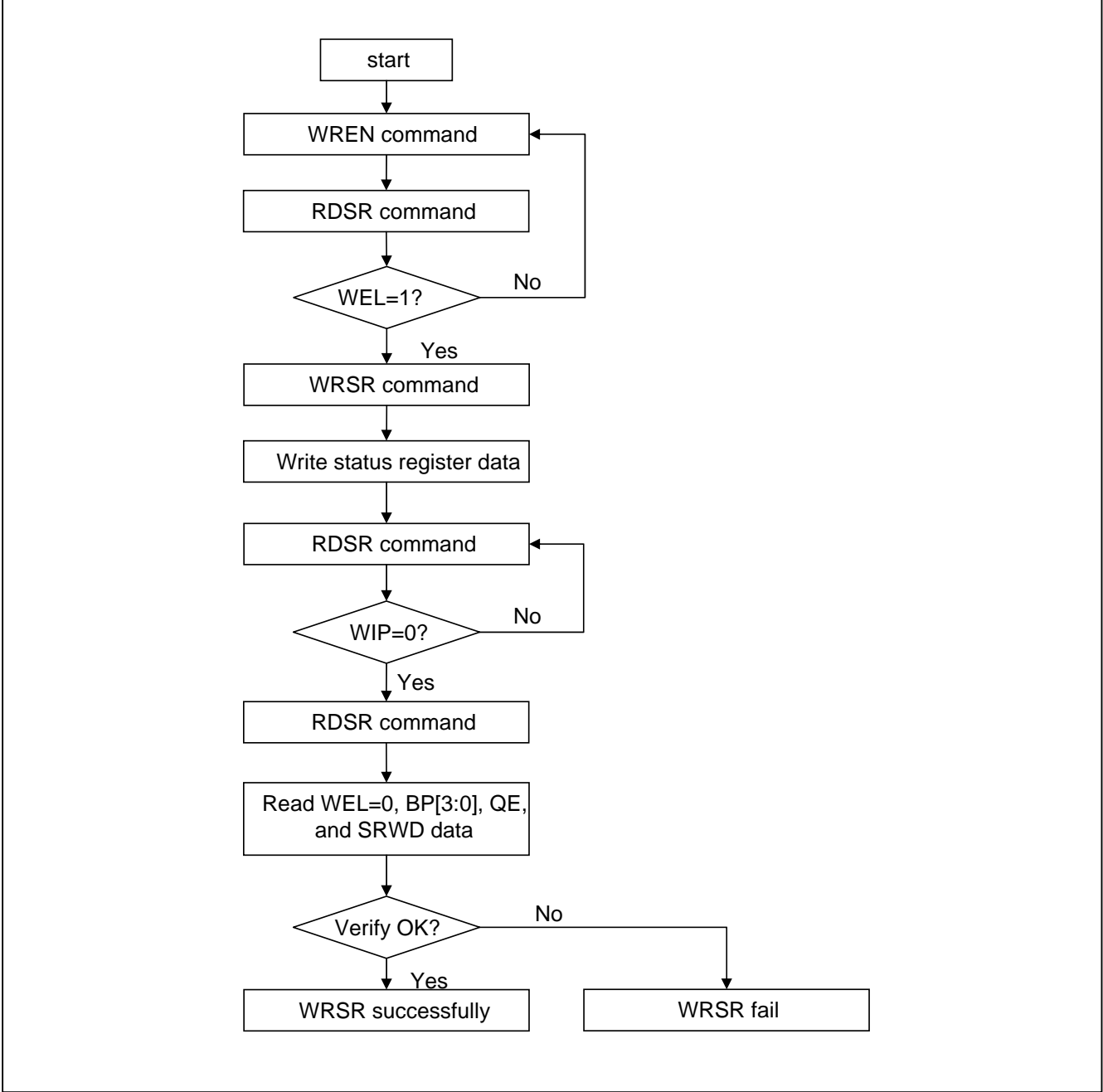
Figure 9. WRSR flow
