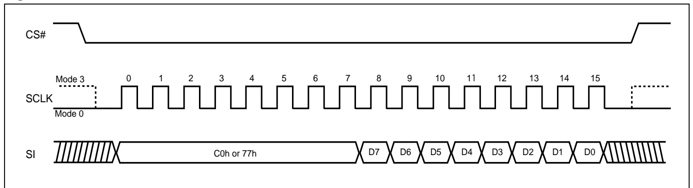
Figure 17. Burst Read
