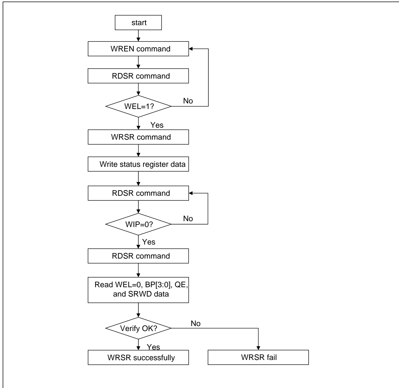
Figure 24. WRSR flow
