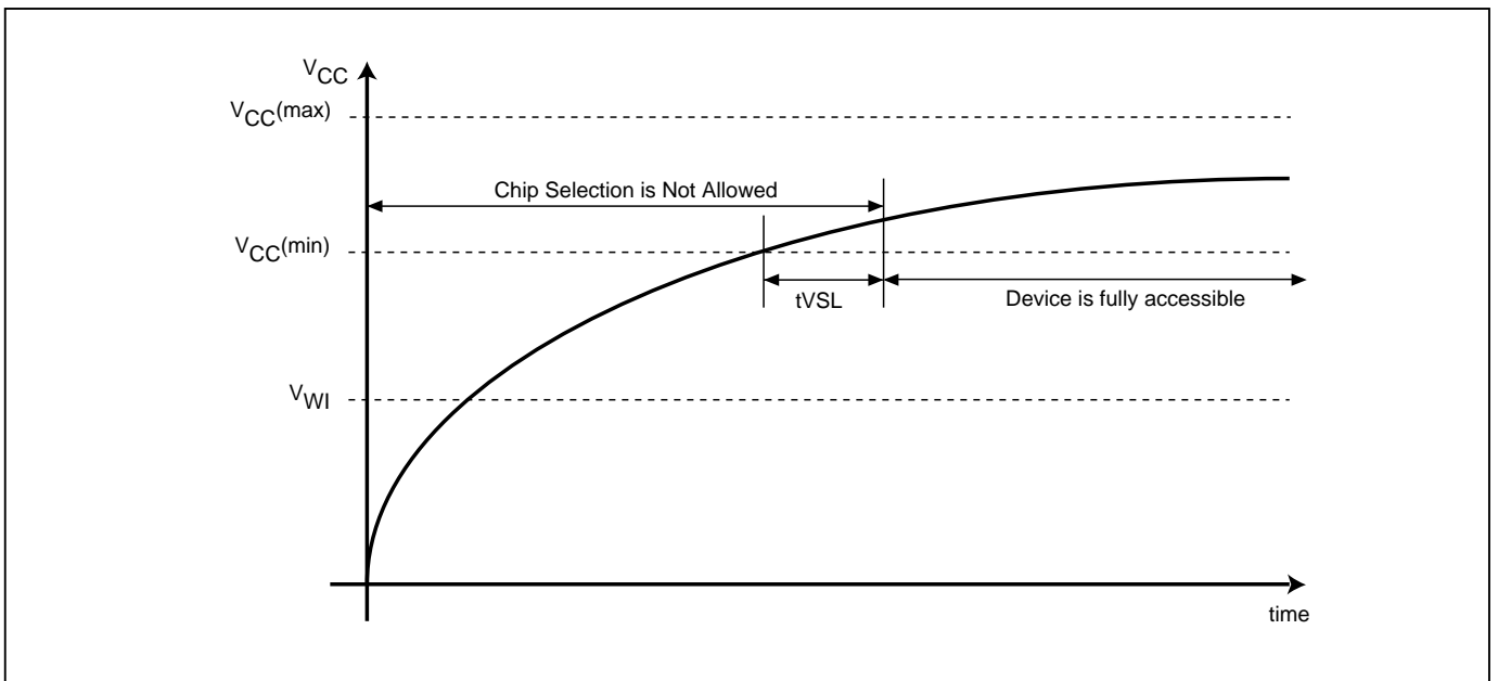
Figure 92. Power-up Timing
