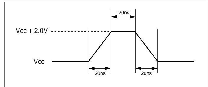
Figure 86. Maximum Positive Overshoot Waveform
