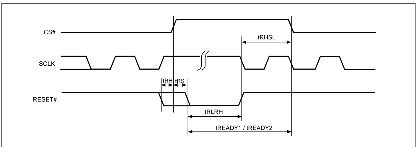
Figure 84. RESET Timing
