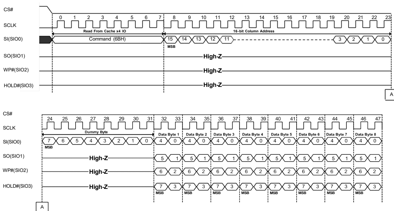
Figure 6-5. Read from Cache x4 IO (6BH) Sequence Diagram
