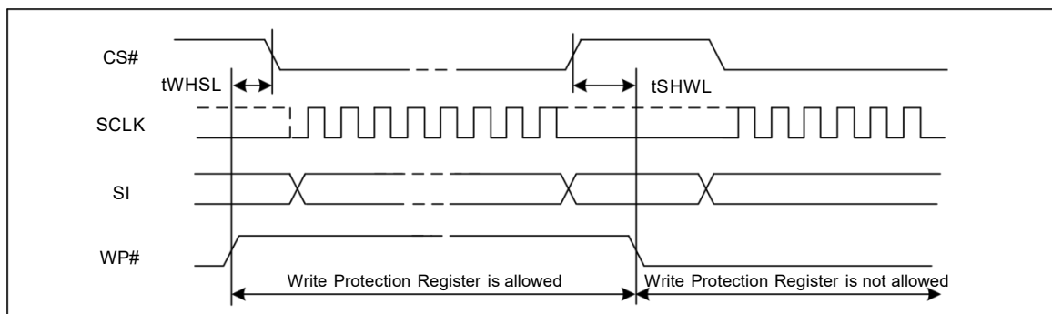
Figure 16-4. WP# Timing
