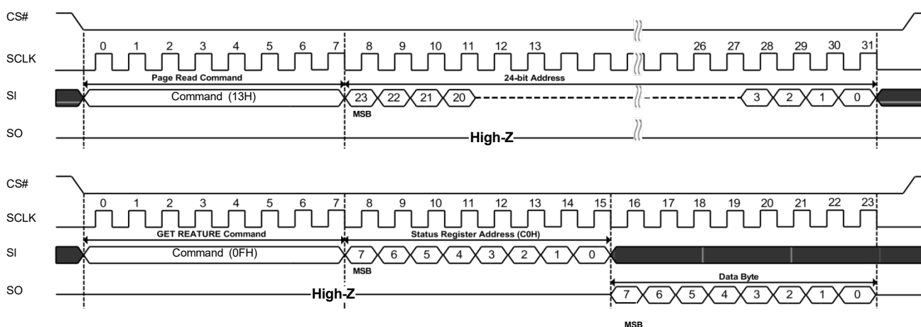
Figure 6-2. Page Read to Cache (13H) Sequence Diagram
