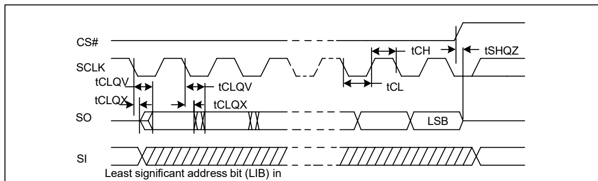
Figure 16-2. Serial Output Timing
