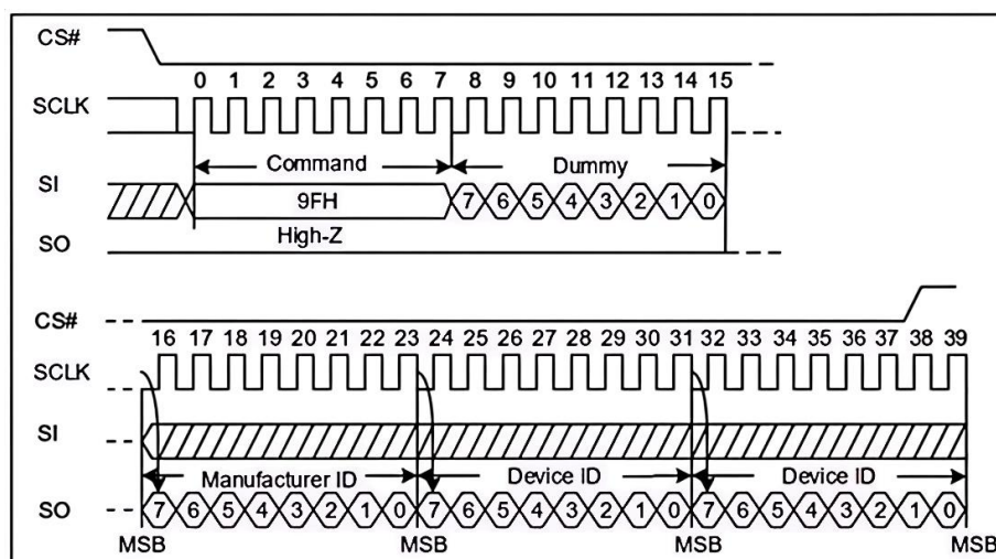
Figure 6-1. Read ID (9FH) Sequence Diagram
