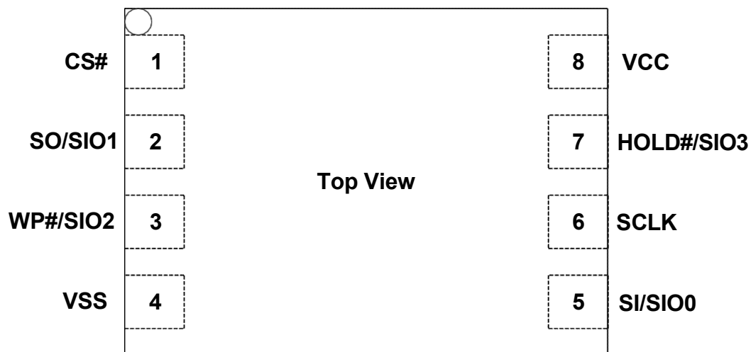
Figure 1-3. Pin Assignments
