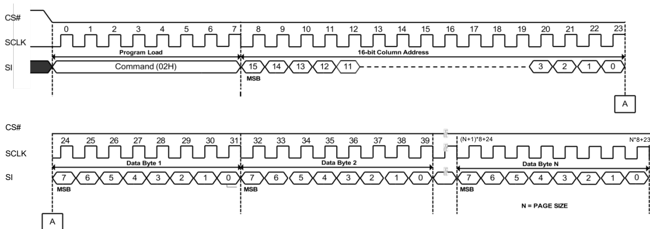
Figure 7-1. Program Load (02H) Sequence Diagram
