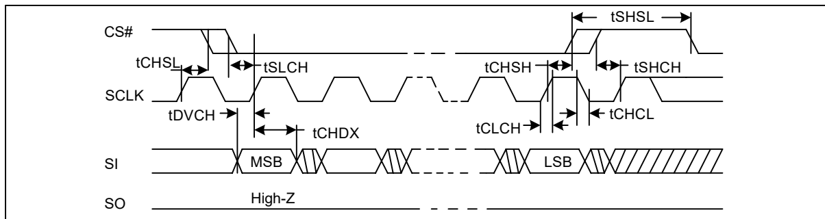
Figure 16-1. Serial Input Timing
