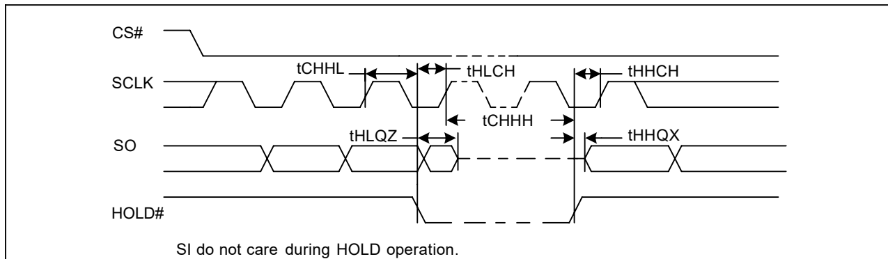
Figure 16-3. Hold# Timing
