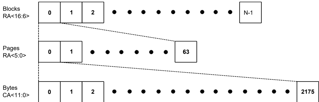
Figure 1-2. Memory Mapping Diagram for 2176 Page size
